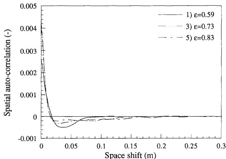
Figure 8. Spatial auto-correlation diagrams of voidage fluctuations (see table 1 for corresponding operating conditions).
