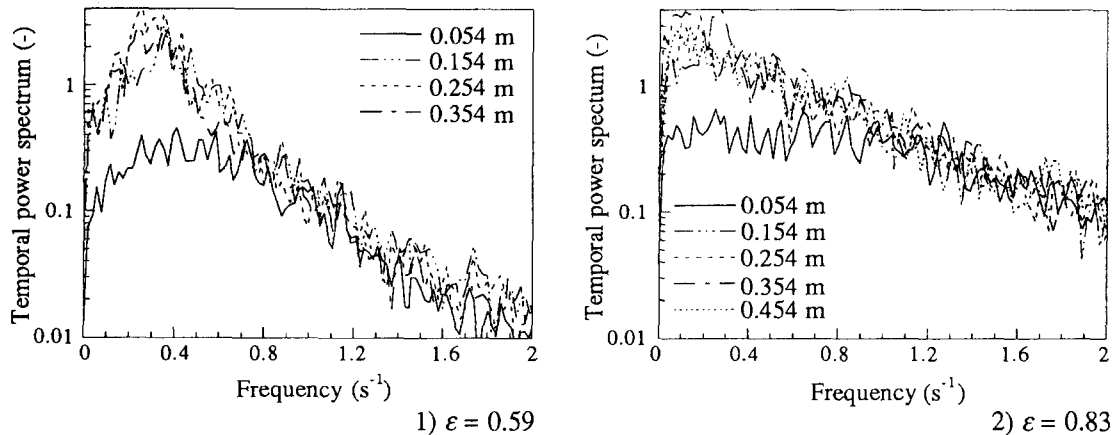
Figure 7. Temporal power spectra at different heights above the distributor (see table 1 for corresponding operating conditions).
