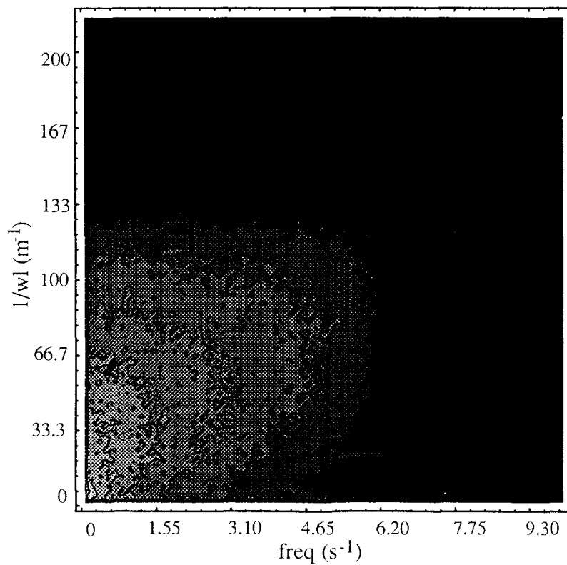
Figure 12. Joint spatial-temporal power spectra (see table 1 for corresponding operating conditions).
