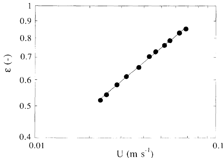
Figure 4. Expansion curve of the bed of spherical particles, d_p = 6.35 \text{ mm} , \rho_p = 1210 \text{ kg m}^{-3} , fluidized with water.
