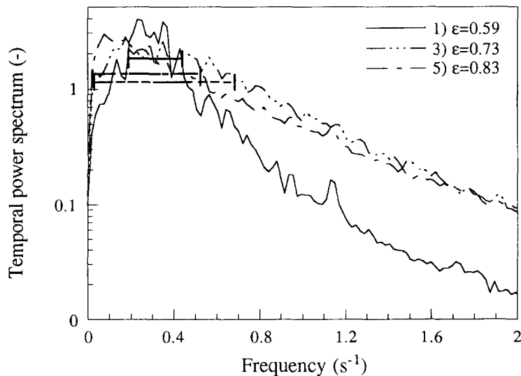
Figure 11. Temporal power spectra (see table 1 for corresponding operating conditions). Horizontal segments indicate more powerful frequencies.
